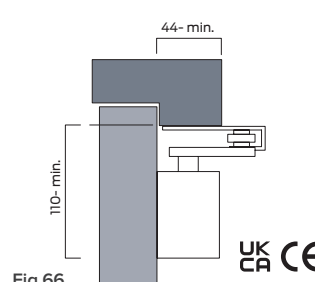
Fig.66 Parallel arm push side mount
