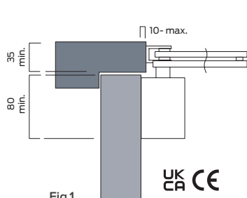
Fig.1 Door mount pull side
