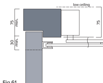
Fig.61 Transom mount push side
